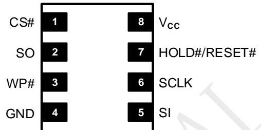
8-Land USON (4x4mm)/WSO (6X5mm)
