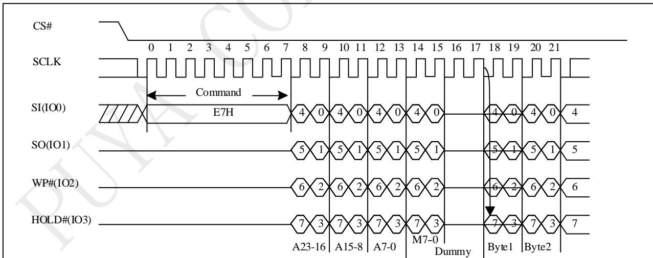
Figure 10-214IO Word Read Sequence (M5-4 \neq (1,0))
