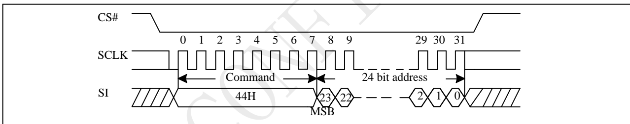
Figure 10-40 Erase Security Registers (ERSCUR) Sequence (Command 44)
