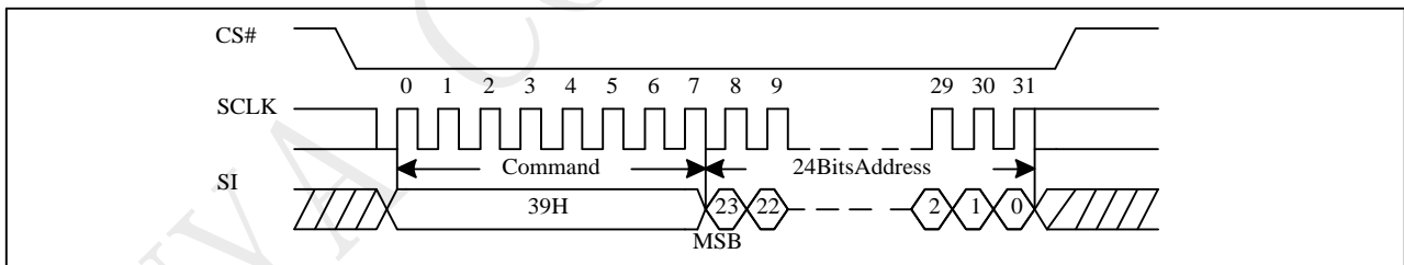
Figure 10-54 Individual Block Unlock (Command 39h)
