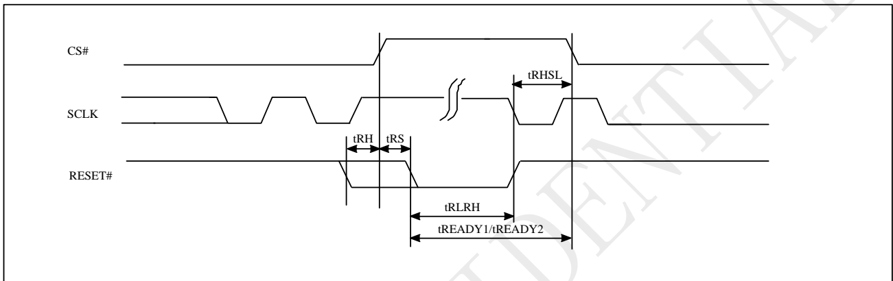
Figure 10-59 RESET Timing
