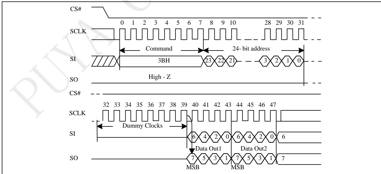
Figure 10-14 Dual Read Mode Sequence (Command 3Bh)
