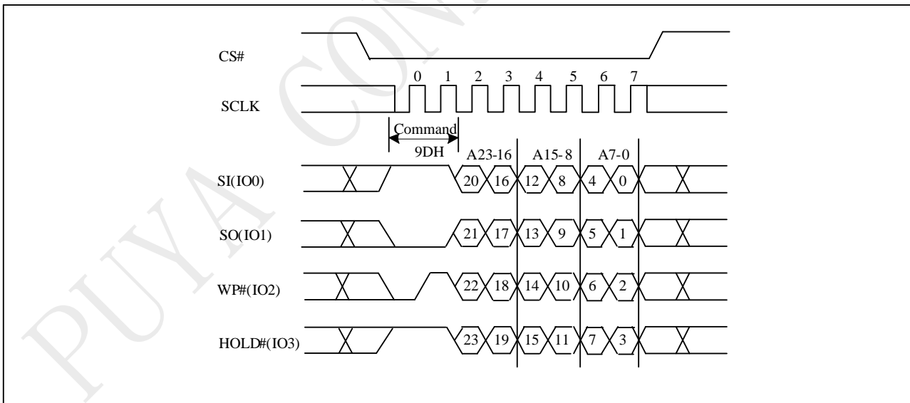
Figure 10-39aBuffer to Main Memory Page Program Sequence (QPI)
